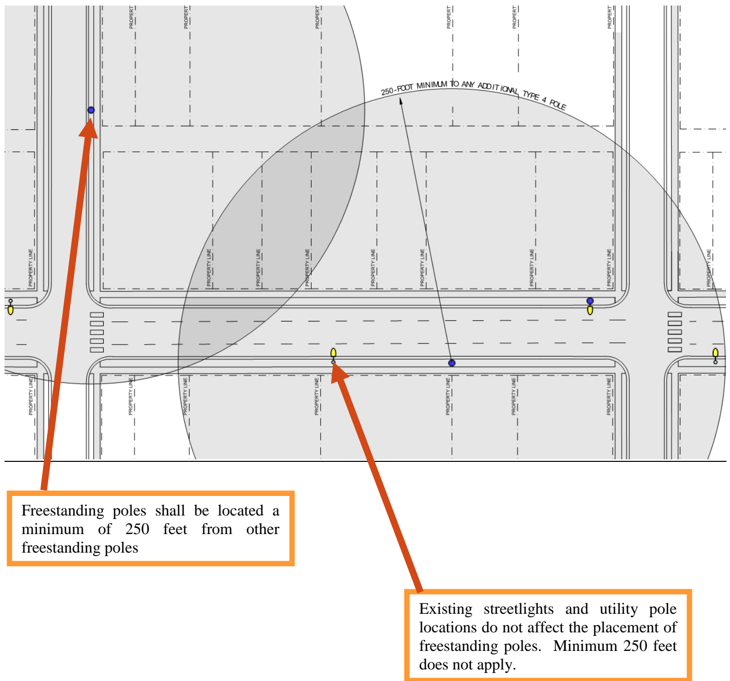
Figure 5.1 – Freestanding Small Cell Spacing Radius
