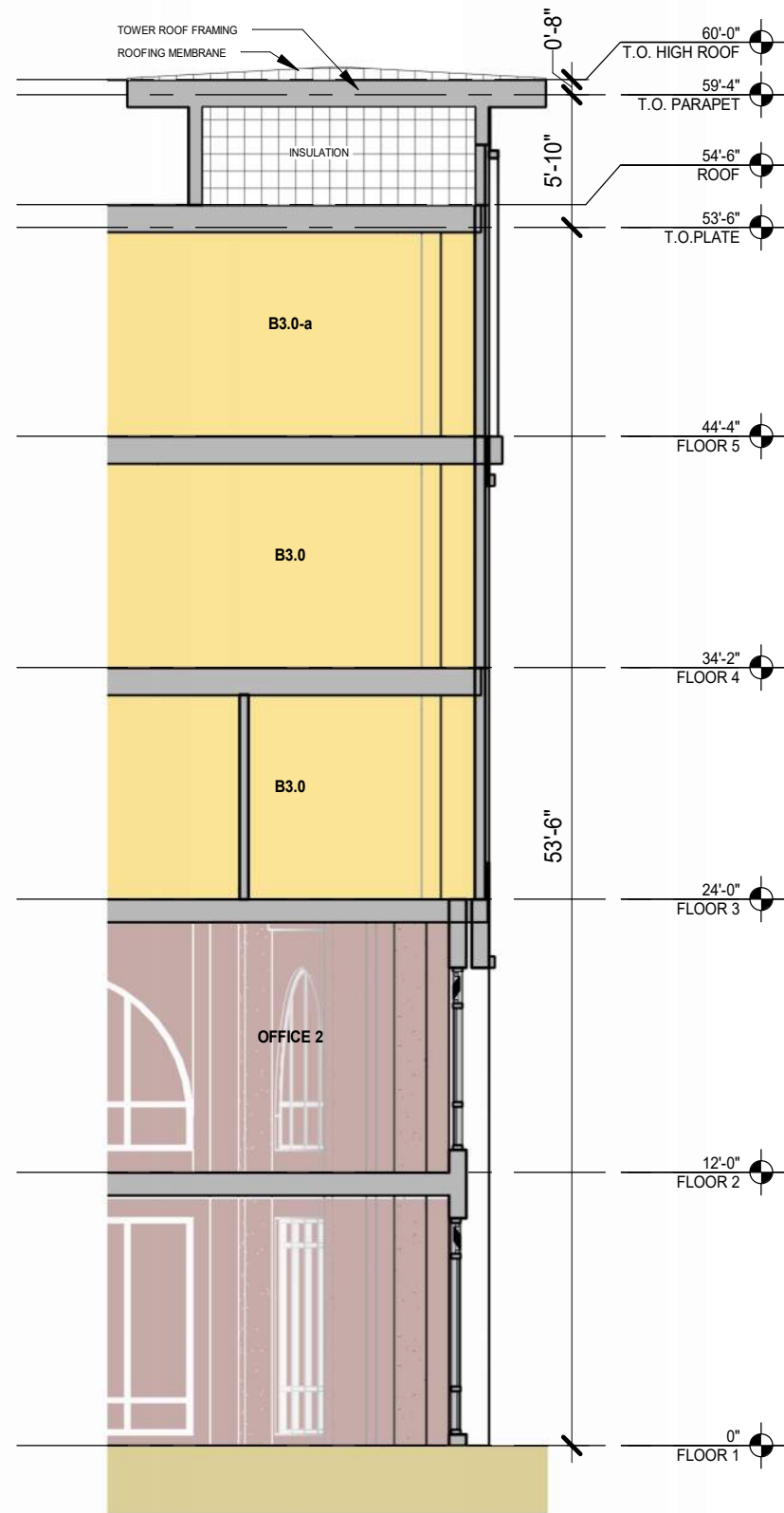
WALL SECTION 2 2
