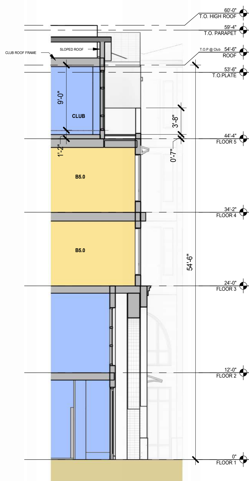
WALL SECTION 1 1
