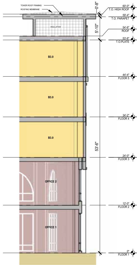
WALL SECTION 2 2
