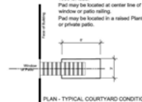
PLAN - TYPICAL COURTYARD CONDITION
