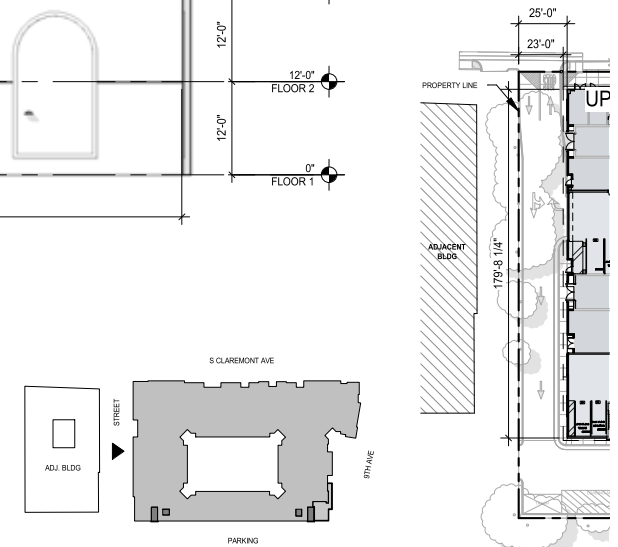
FLOOR 1- PARTIAL WEST SITE PLAN 1
