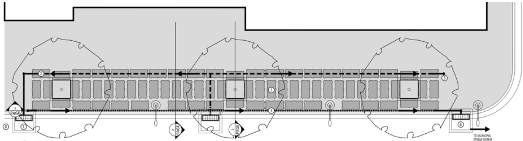
SILVA CELL SYSTEM + CATCH BASIN
