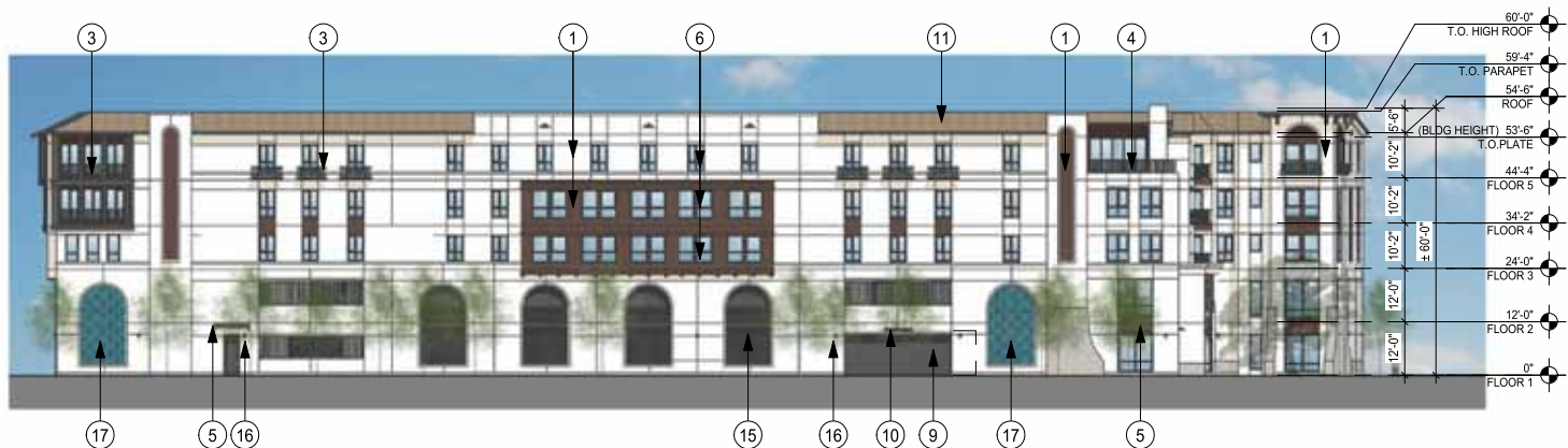
ELEVATION - SOUTH 2
