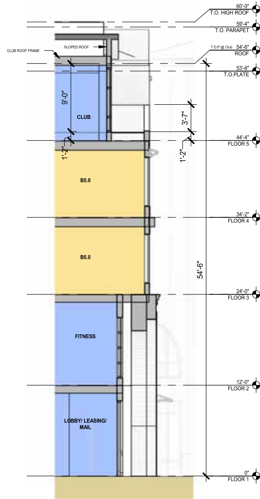
WALL SECTION 1 1
