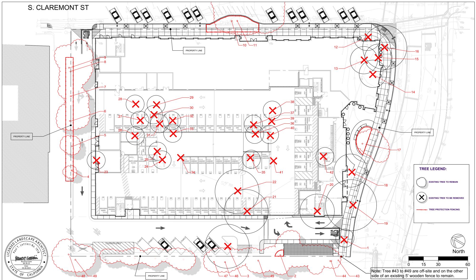
TREE DISPOSITION PLAN L-5.1
