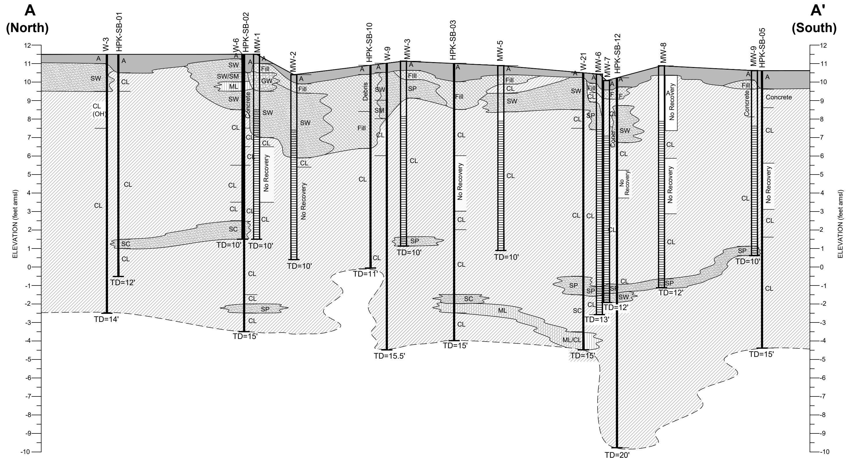
Figure 8 Cross Section A-A' Hayward Park Caltrain Station San Mateo, California
