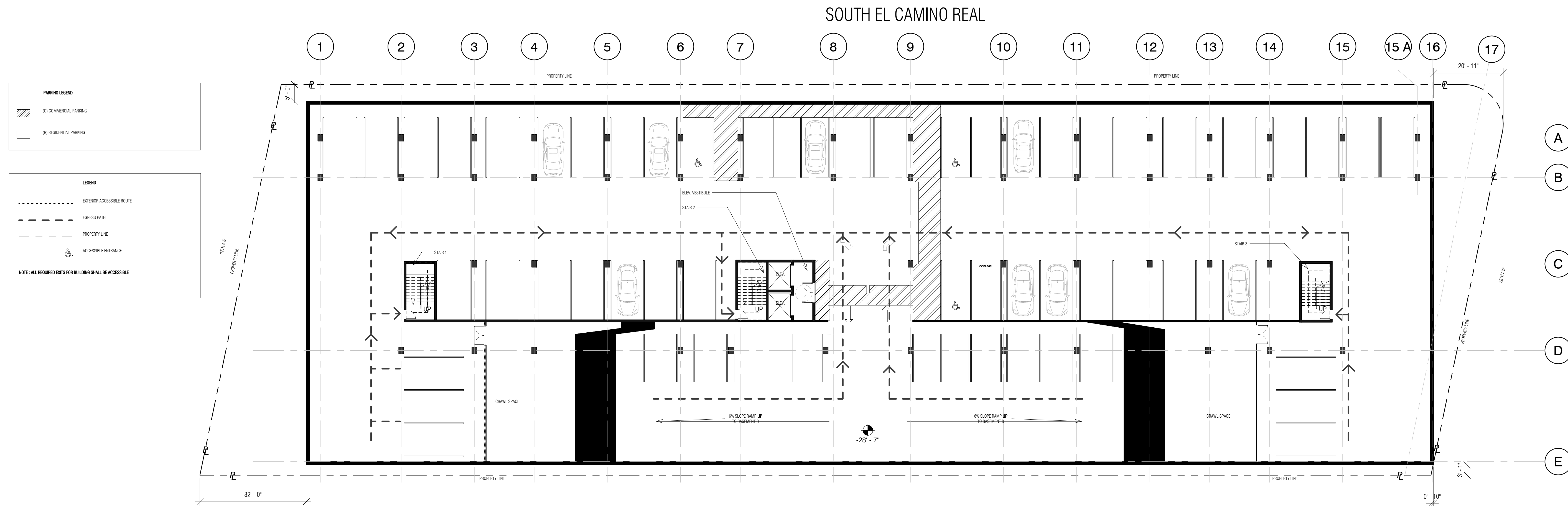
2 Basement Level C - Residential Parking - Egress 1/16" = 1'-0"
