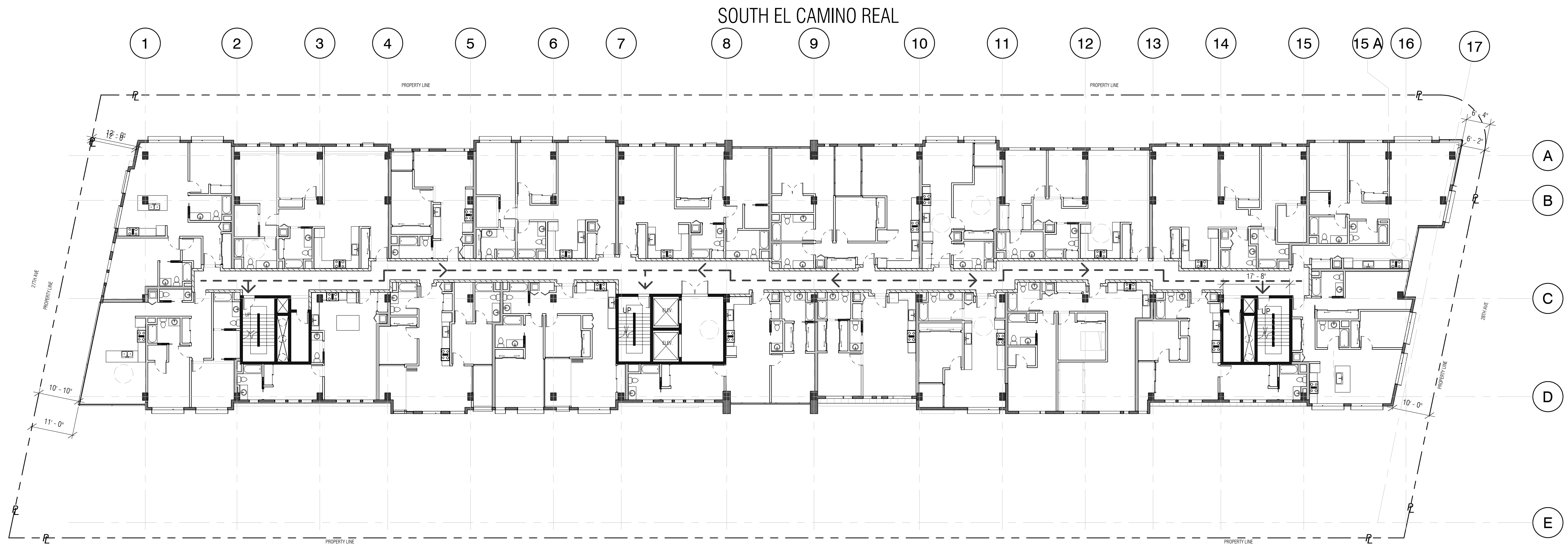
2 Level 3 - Egress 1/16" = 1'-0"
